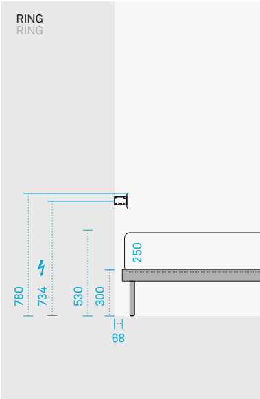
L 2600 H 780 P 2200 Barnum 13, Grafite, Noce W 2600 H 780 D 2200 Barnum 13, Grafite, Walnut
