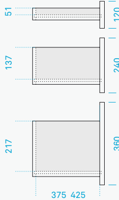
VISTA LATERALE SIDE VIEW
