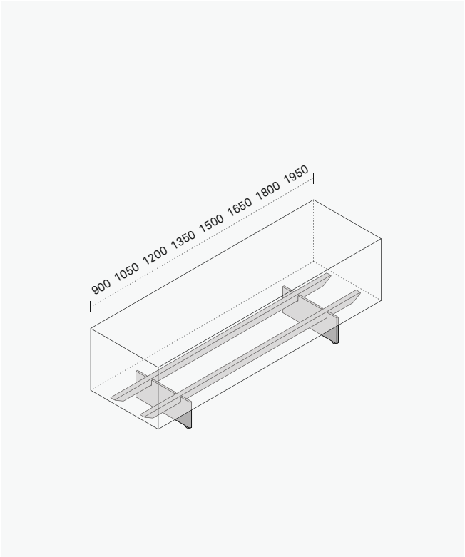
A due appoggi. With two supports.
