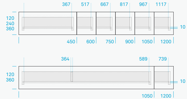
VISTA FRONTALE FRONT VIEW
