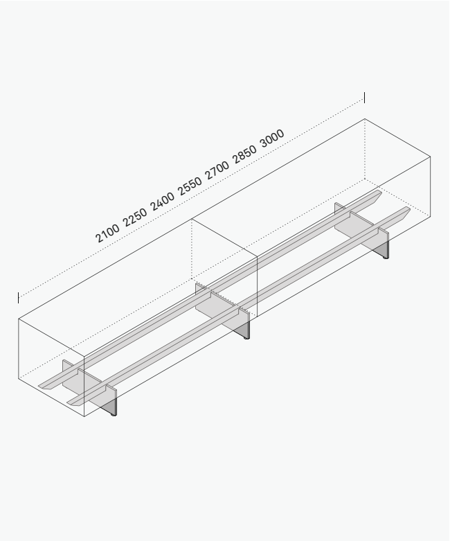
A tre appoggi. With three supports.
