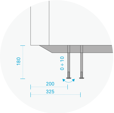
* Per Base bifacciale * For double-sided Base * Battiscopa * Skirting board
