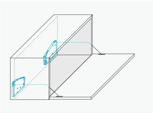
Ribalta inferiore Lower flap door
