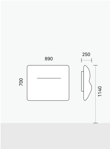
Schienale tessile R Upholstered back panel R
