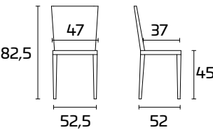
Daydream 401 Daydream 401 transparent (cantilever)
