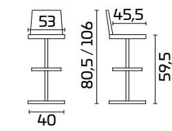
Gliss with height-adjustable revolving seat
