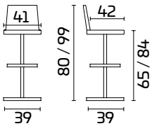
Flash with height-adjustable revolving seat
