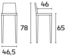
Cantilever leg Freesby
