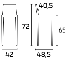
Endless straight leg
