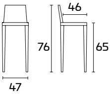
Straight leg Freesby
