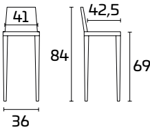
Flash with fixed seat
