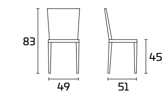
Straight leg Hero
